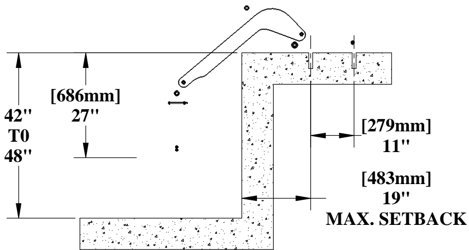
FRONT VIEW (LIFT IN WATER)
